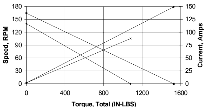
ADL 250 Nominal Speed-Torque Curves
