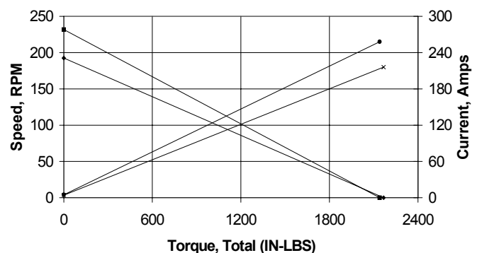
ADL 290 Nominal Speed-Torque Curves
